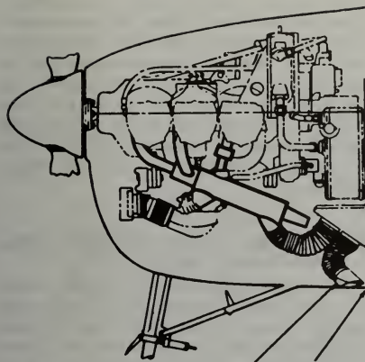
FIGURE 2-28. Exhaust system of a horizontally opposed engine.
